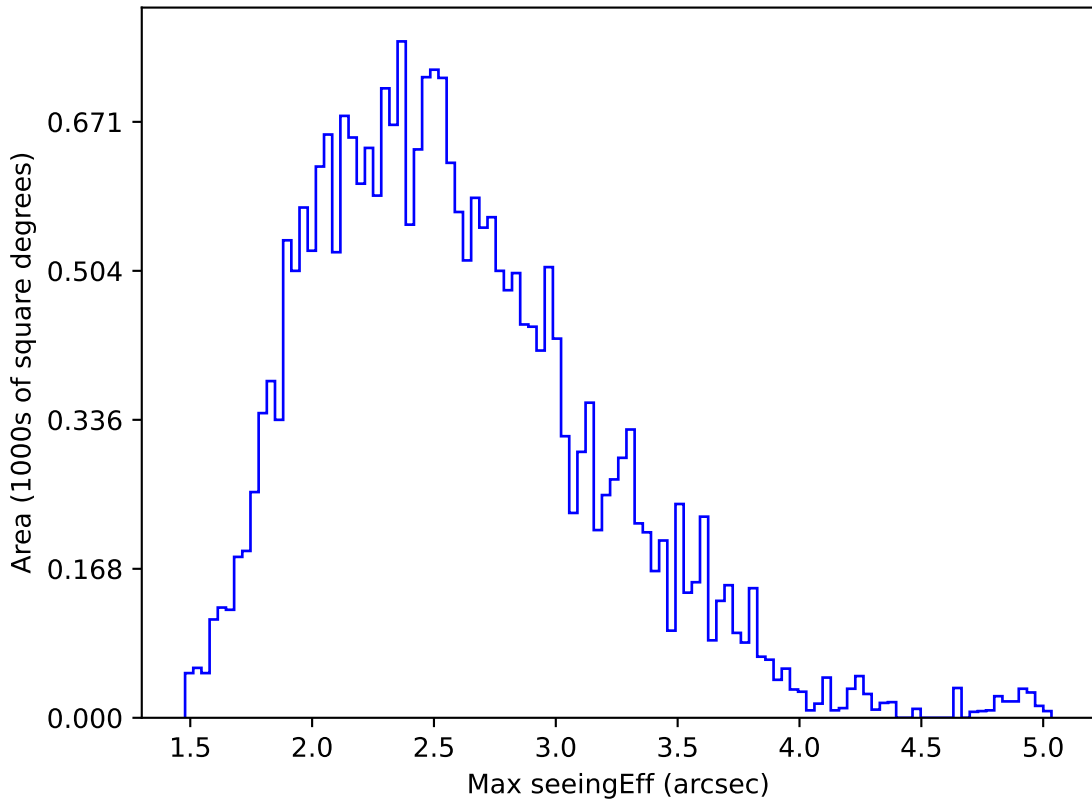
roman_v3.3_10yrs All sky i band: Max seeingEff
