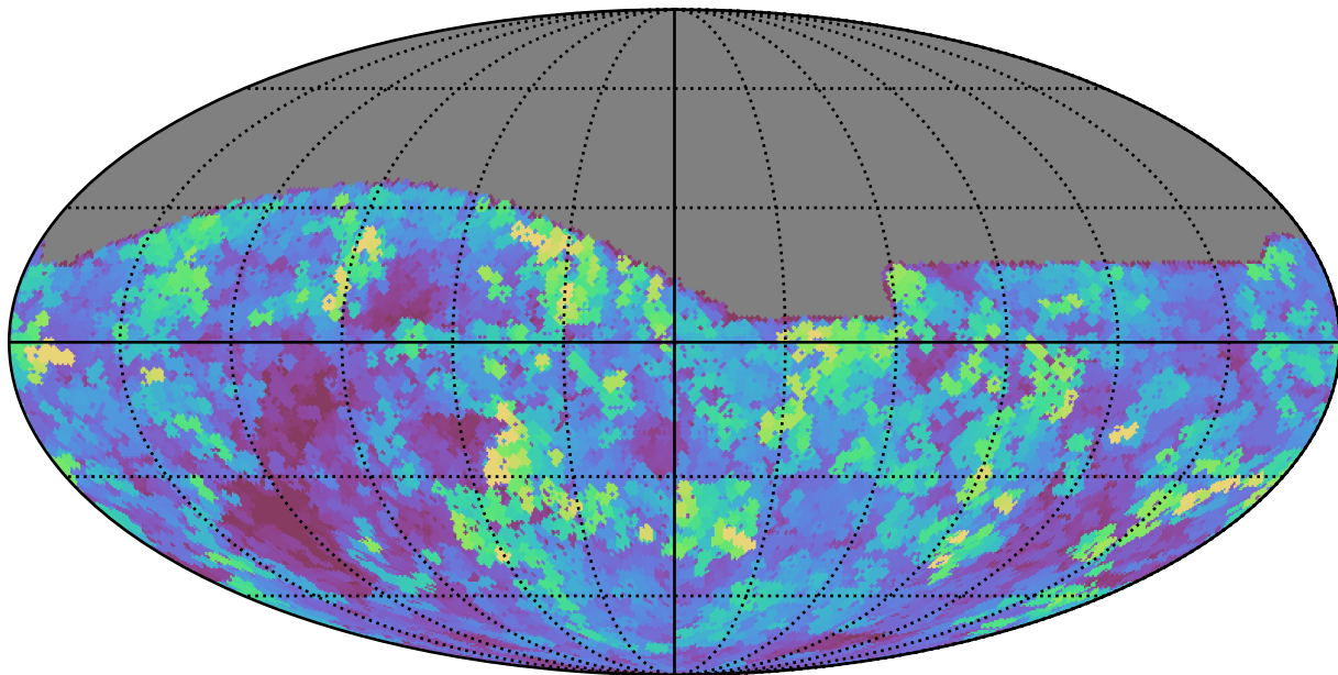
roman_v3.3_10yrs All sky g band: Max seeingEff
