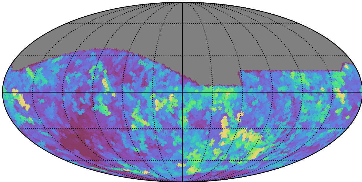
roman_v3.3_10yrs All sky all bands: Max seeingEff
