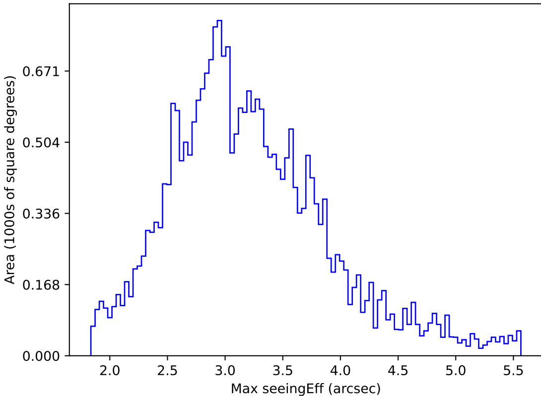
roman_v3.3_10yrs All sky all bands: Max seeingEff
