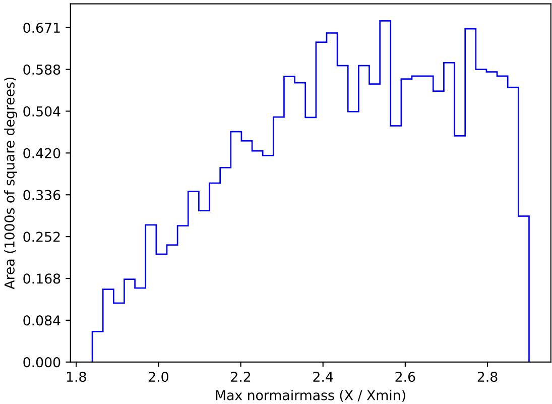
roman_v3.3_10yrs WFD all bands: Max normairmass
