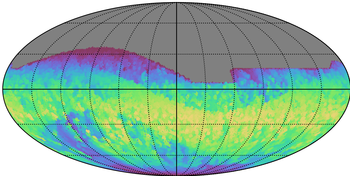
roman_v3.3_10yrs All sky all bands: Max normairmass
