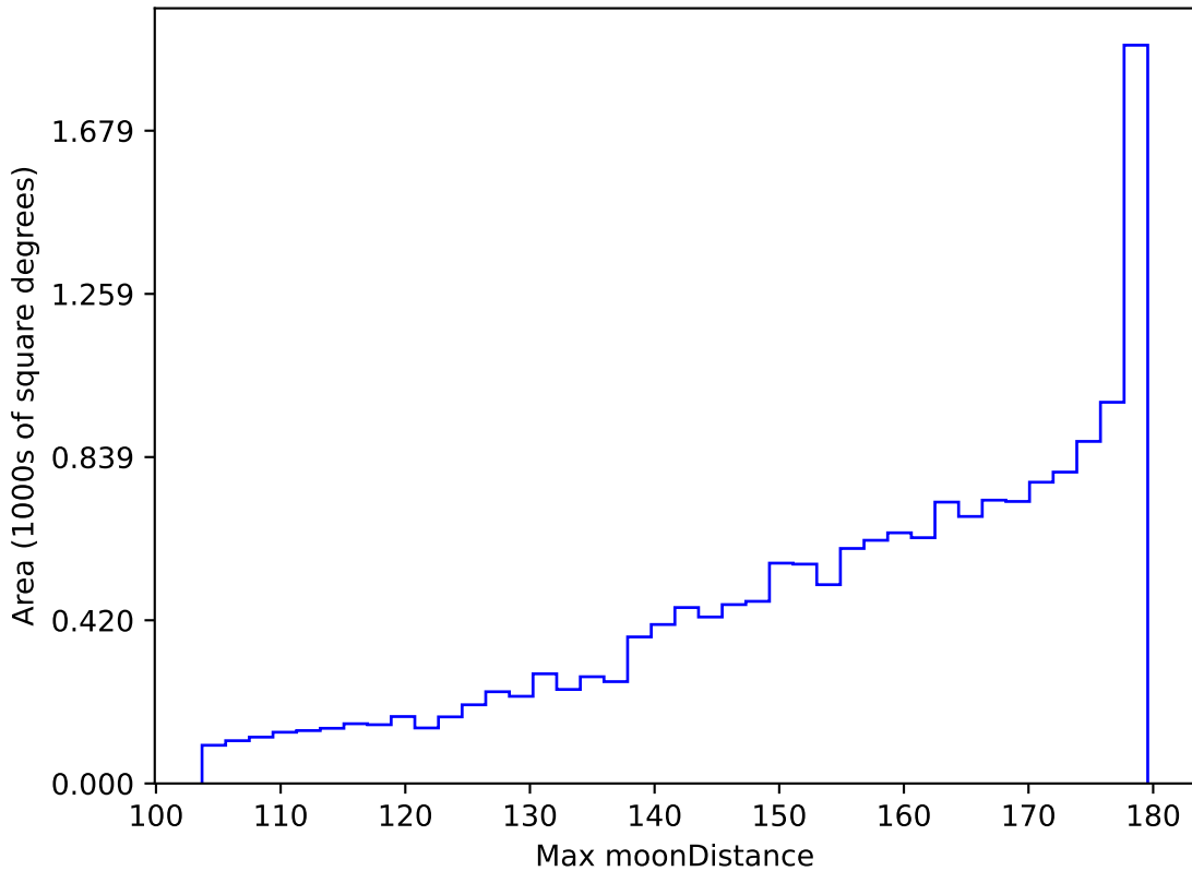
roman_v3.3_10yrs WFD all bands: Max moonDistance
