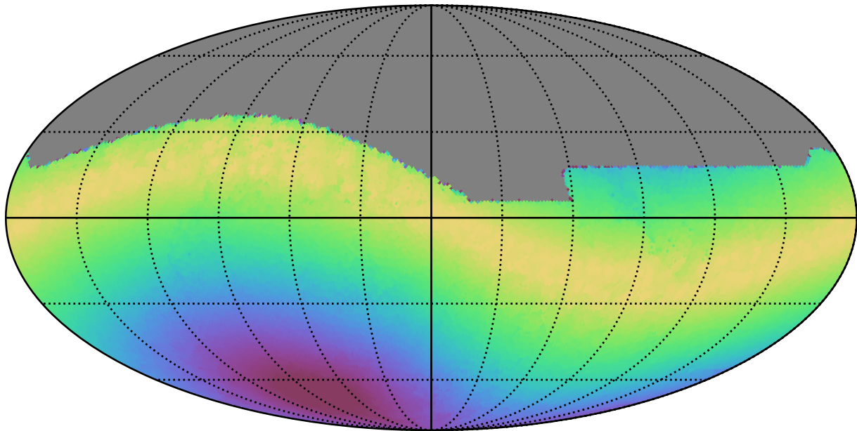
roman_v3.3_10yrs All sky all bands: Max moonDistance
