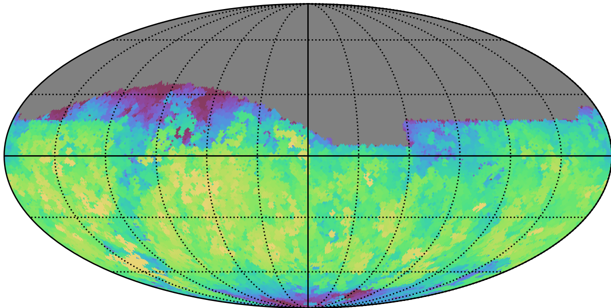
roman_v3.3_10yrs Yr 1 z band: Max fiveSigmaDepth
