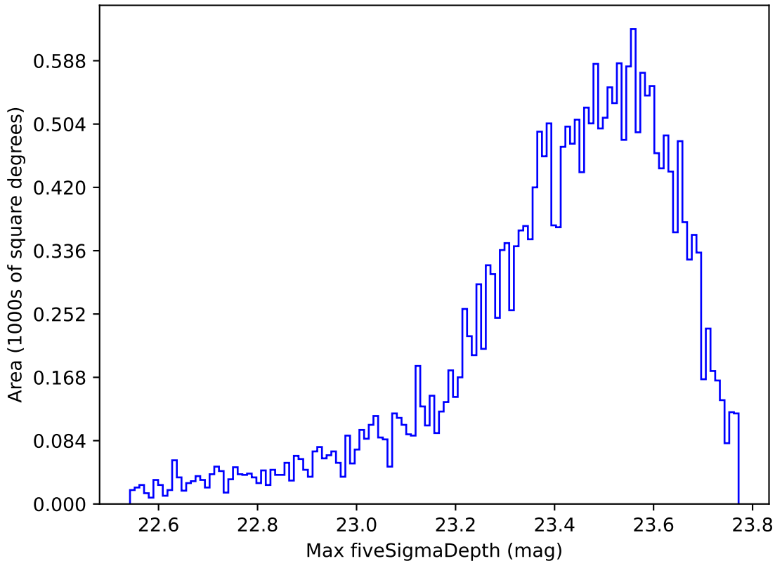
roman_v3.3_10yrs Yr 1 z band: Max fiveSigmaDepth
