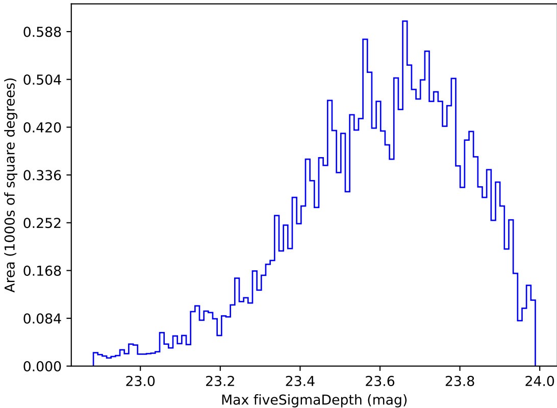
roman_v3.3_10yrs Yr 1 u band: Max fiveSigmaDepth
