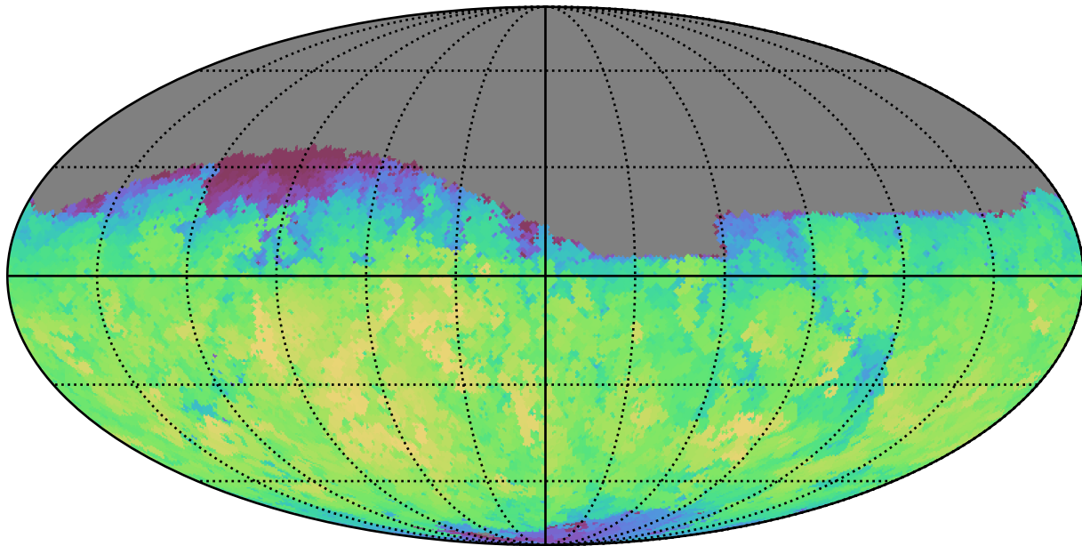
roman_v3.3_10yrs Yr 1 r band: Max fiveSigmaDepth
