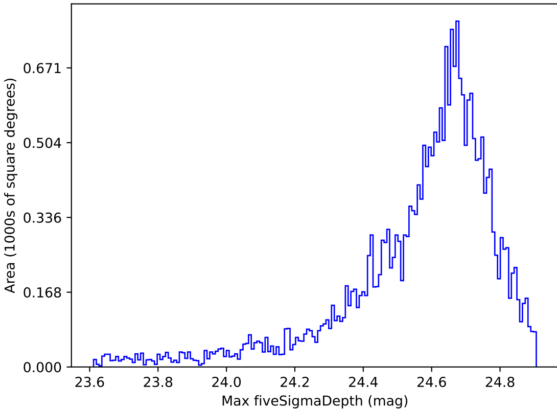
roman_v3.3_10yrs Yr 1 r band: Max fiveSigmaDepth
