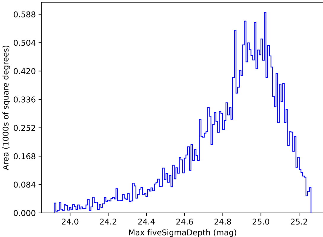
roman_v3.3_10yrs Yr 1 g band: Max fiveSigmaDepth
