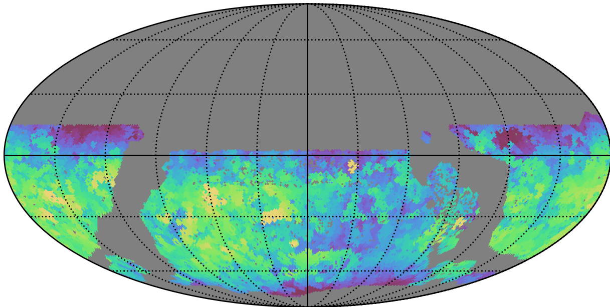
roman_v3.3_10yrs WFD u band: Max fiveSigmaDepth
