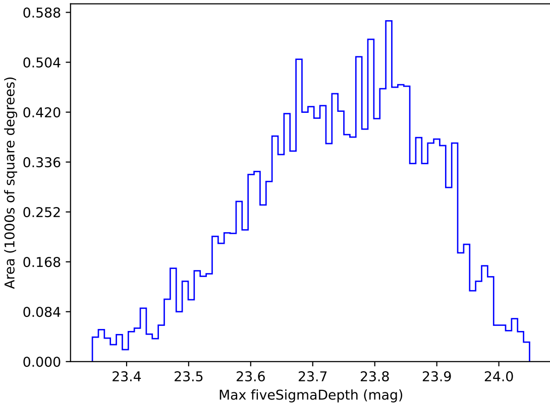
roman_v3.3_10yrs WFD u band: Max fiveSigmaDepth
