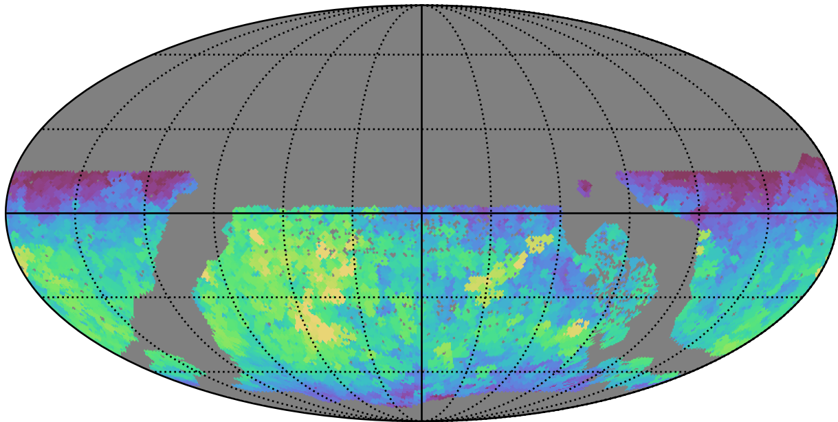
roman_v3.3_10yrs WFD r band: Max fiveSigmaDepth
