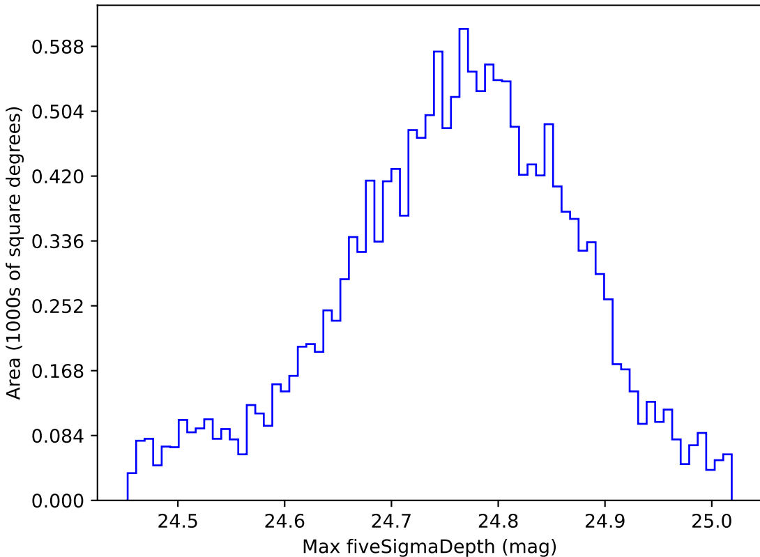
roman_v3.3_10yrs WFD r band: Max fiveSigmaDepth
