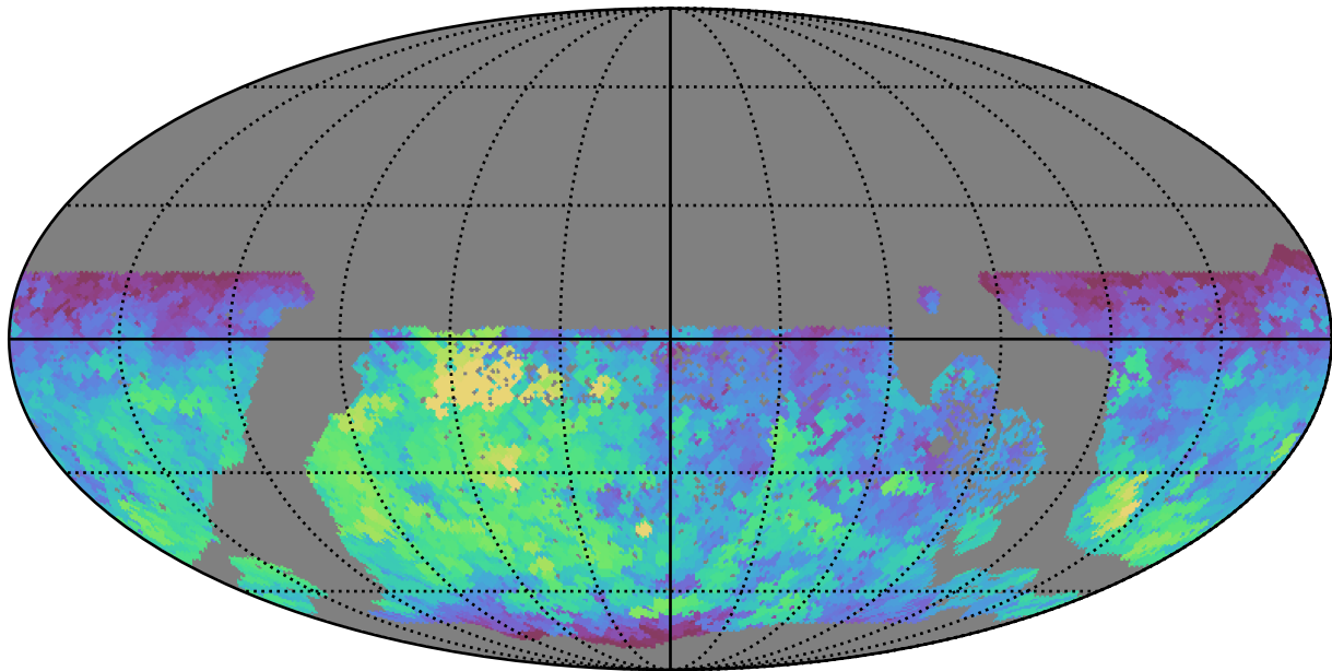
roman_v3.3_10yrs WFD all bands: Max fiveSigmaDepth
