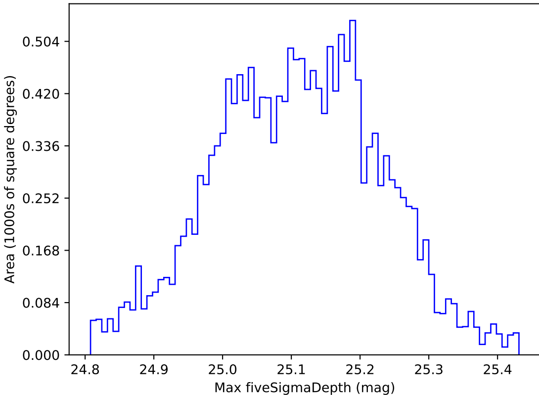
roman_v3.3_10yrs WFD all bands: Max fiveSigmaDepth
