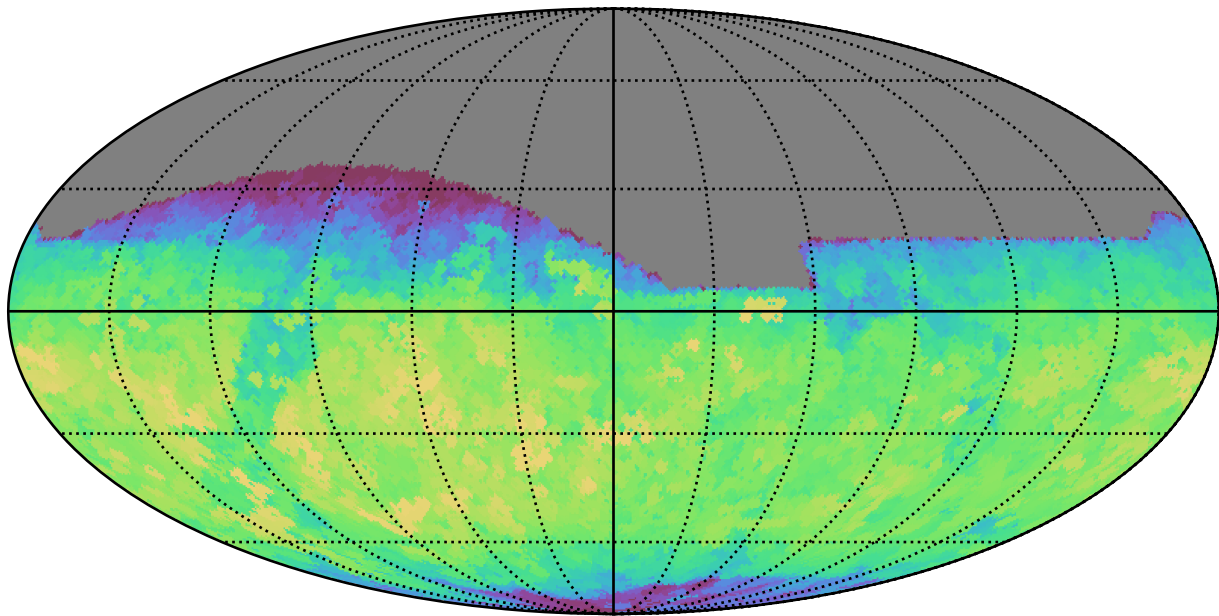
roman_v3.3_10yrs All sky z band: Max fiveSigmaDepth
