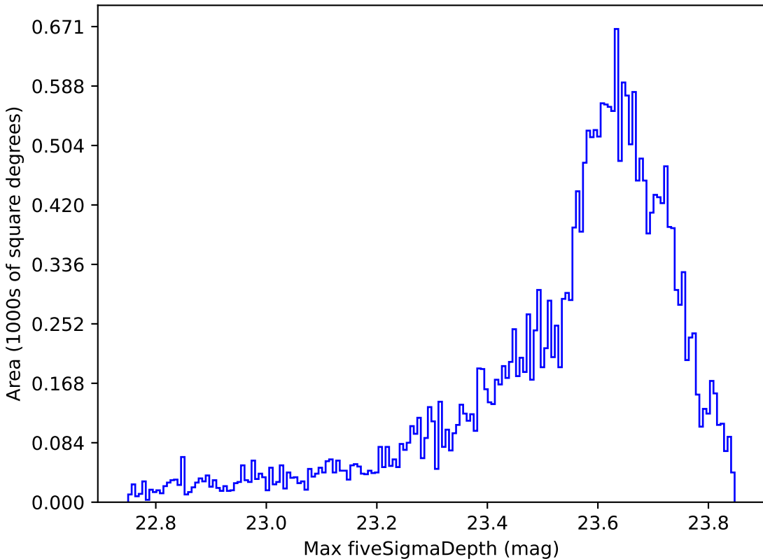
roman_v3.3_10yrs All sky z band: Max fiveSigmaDepth
