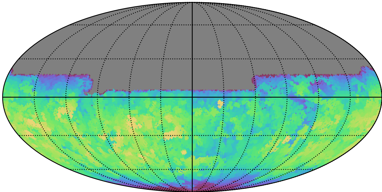
roman_v3.3_10yrs All sky u band: Max fiveSigmaDepth
