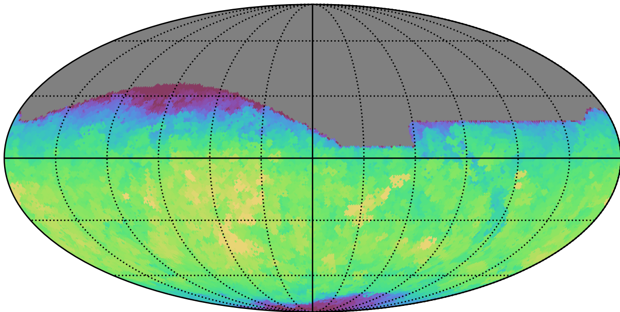
roman_v3.3_10yrs All sky r band: Max fiveSigmaDepth
