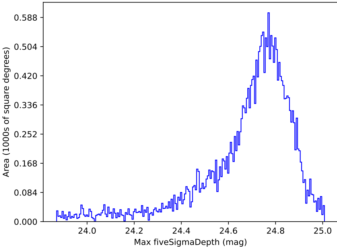
roman_v3.3_10yrs All sky r band: Max fiveSigmaDepth
