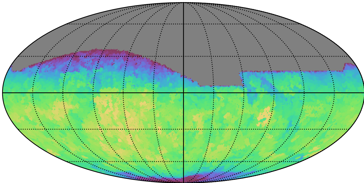
roman_v3.3_10yrs All sky i band: Max fiveSigmaDepth
