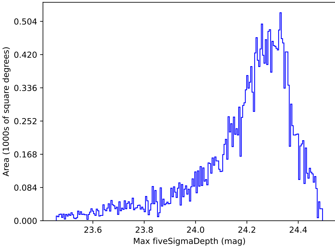
roman_v3.3_10yrs All sky i band: Max fiveSigmaDepth
