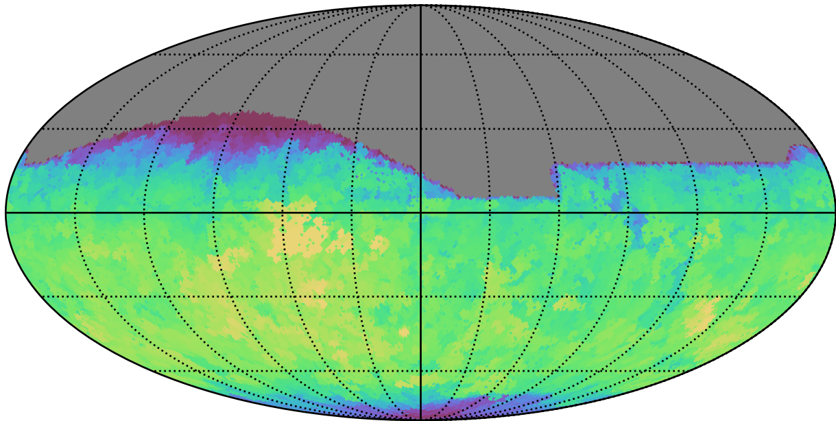
roman_v3.3_10yrs All sky g band: Max fiveSigmaDepth
