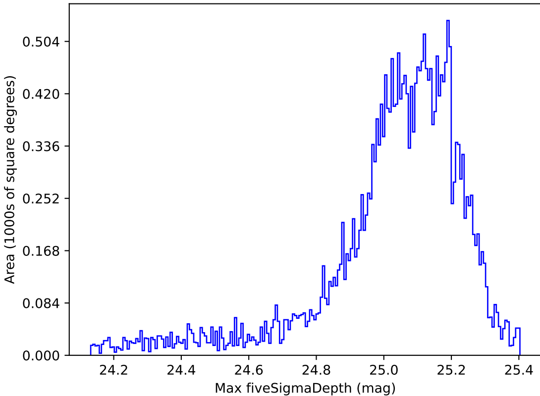
roman_v3.3_10yrs All sky g band: Max fiveSigmaDepth
