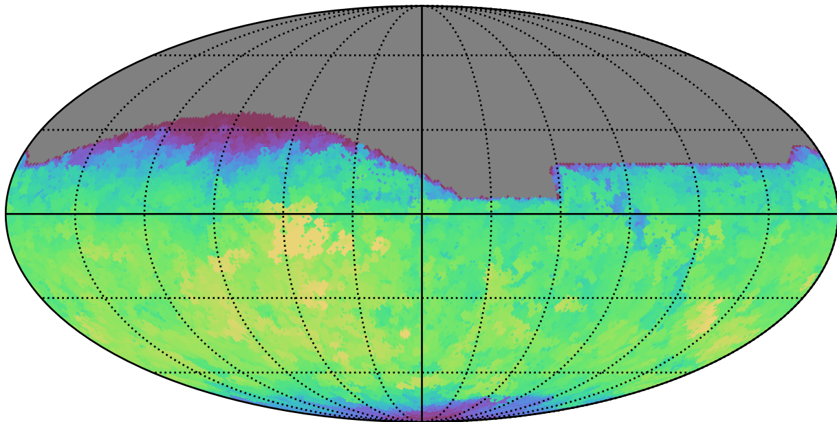
roman_v3.3_10yrs All sky all bands: Max fiveSigmaDepth
