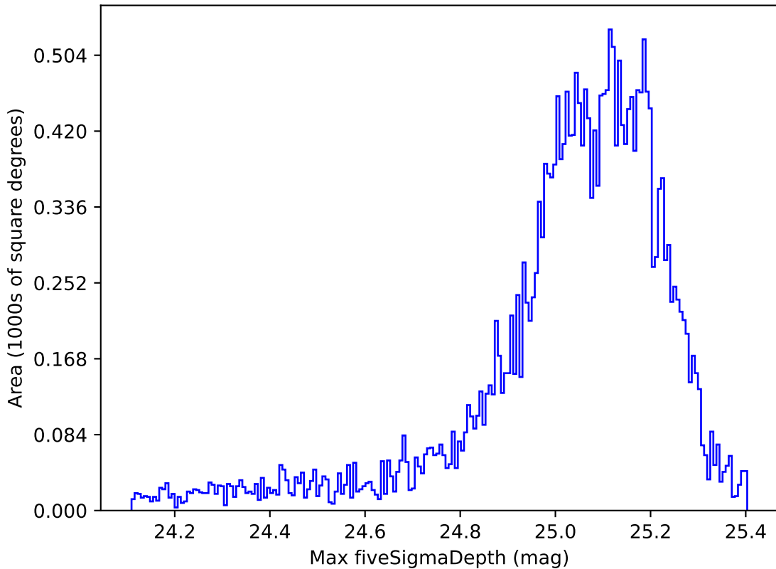
roman_v3.3_10yrs All sky all bands: Max fiveSigmaDepth
