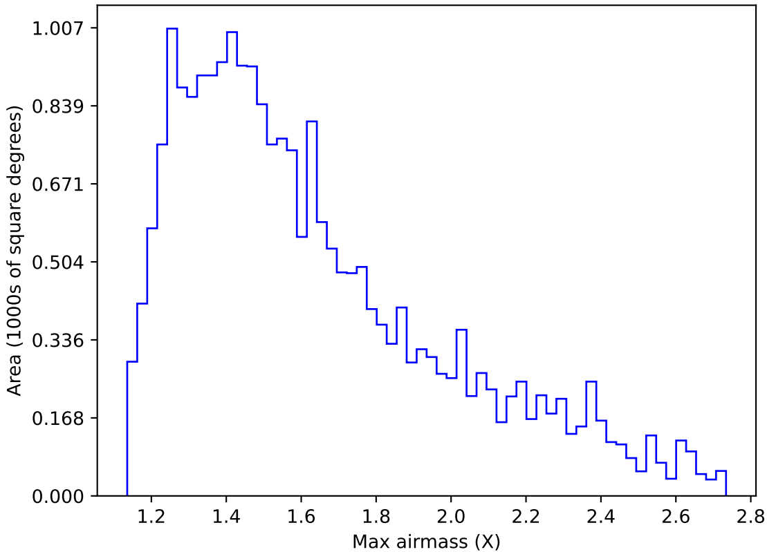
roman_v3.3_10yrs Yr 1 y band: Max airmass
