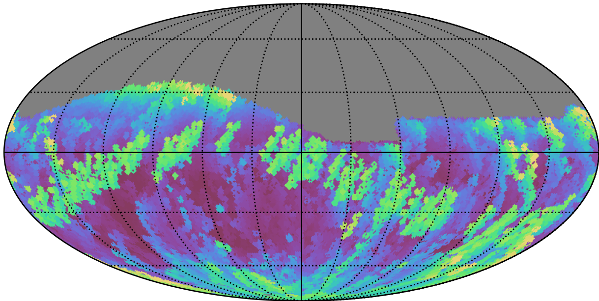
roman_v3.3_10yrs Yr 1 r band: Max airmass
