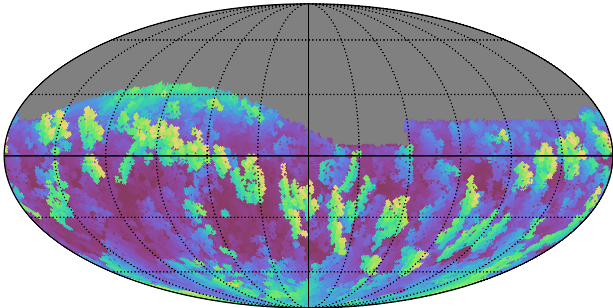
roman_v3.3_10yrs Yr 1 i band: Max airmass
