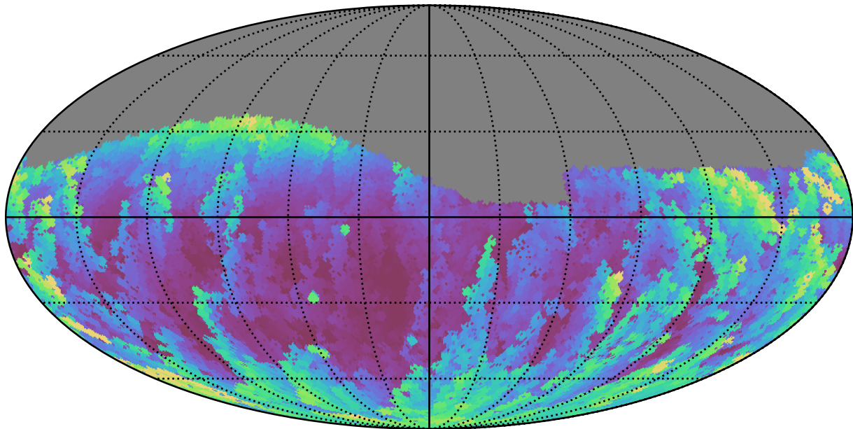
roman_v3.3_10yrs Yr 1 g band: Max airmass
