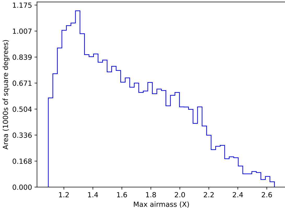
roman_v3.3_10yrs Yr 1 g band: Max airmass
