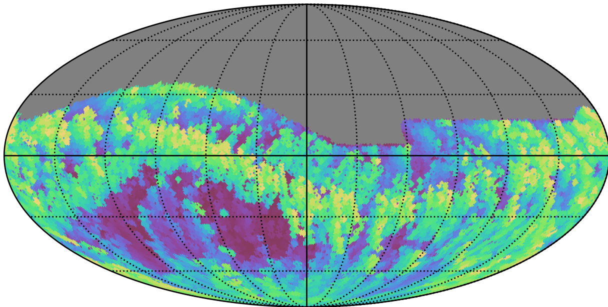
roman_v3.3_10yrs Yr 1 all bands: Max airmass
