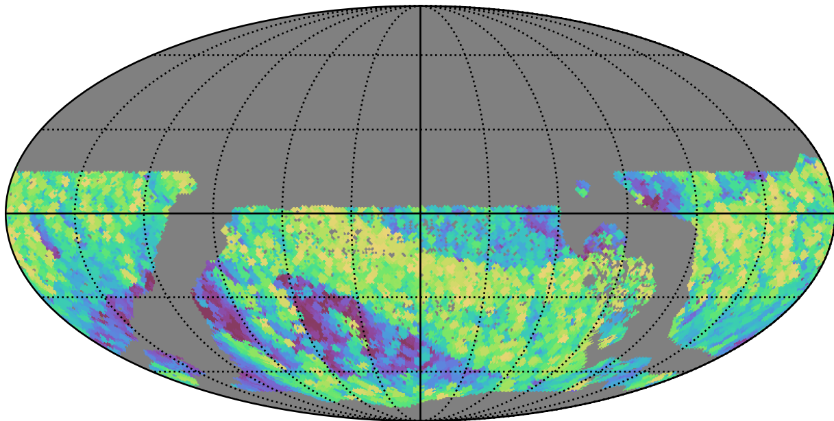
roman_v3.3_10yrs WFD z band: Max airmass
