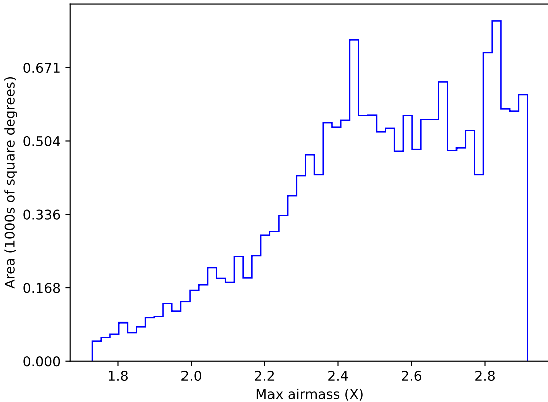
roman_v3.3_10yrs WFD z band: Max airmass
