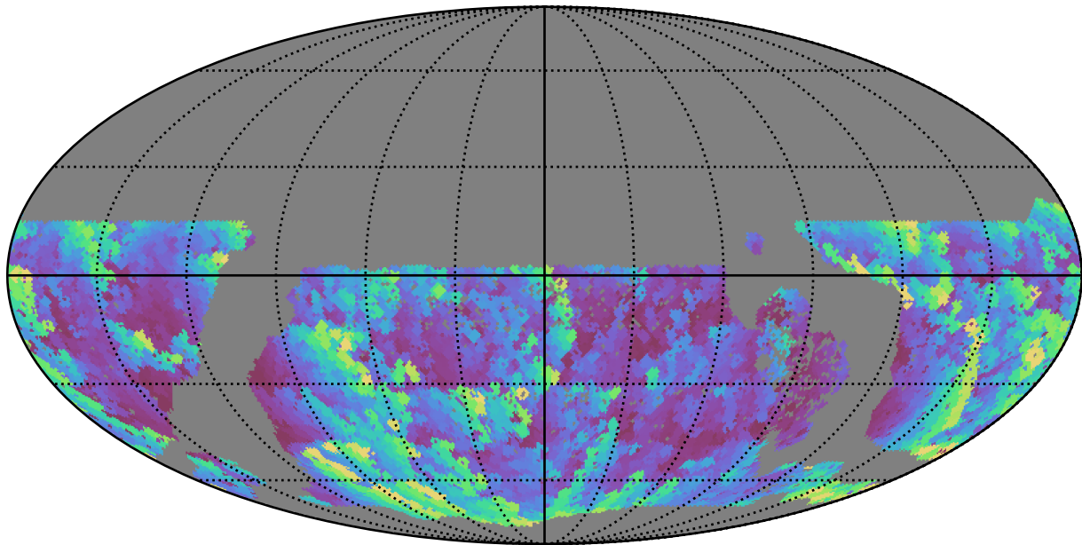
roman_v3.3_10yrs WFD u band: Max airmass
