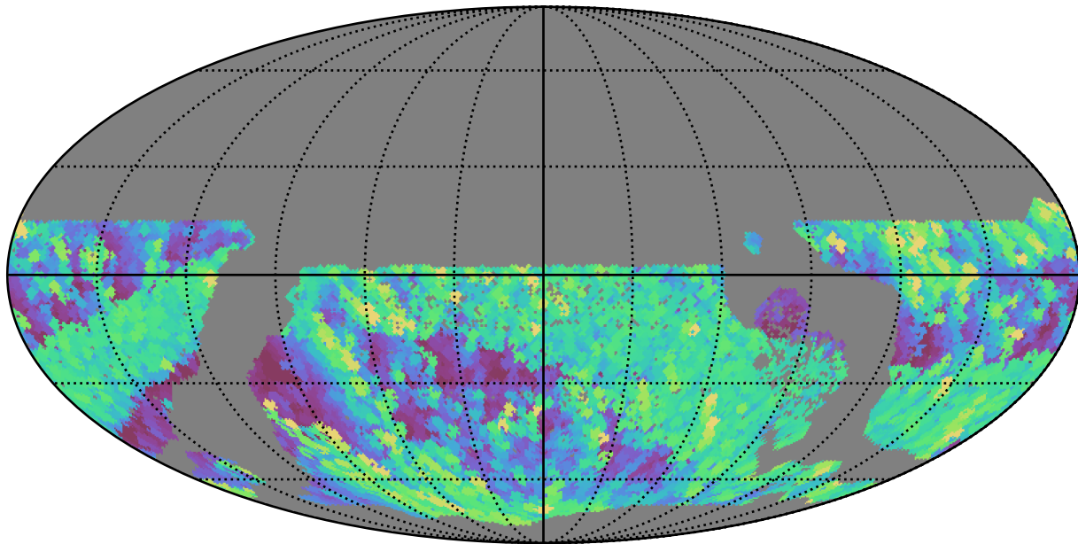
roman_v3.3_10yrs WFD r band: Max airmass
