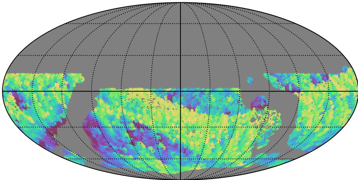
roman_v3.3_10yrs WFD i band: Max airmass
