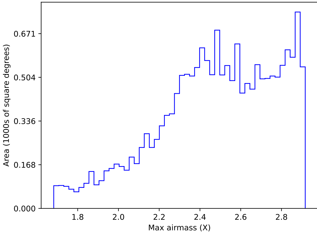
roman_v3.3_10yrs WFD i band: Max airmass
