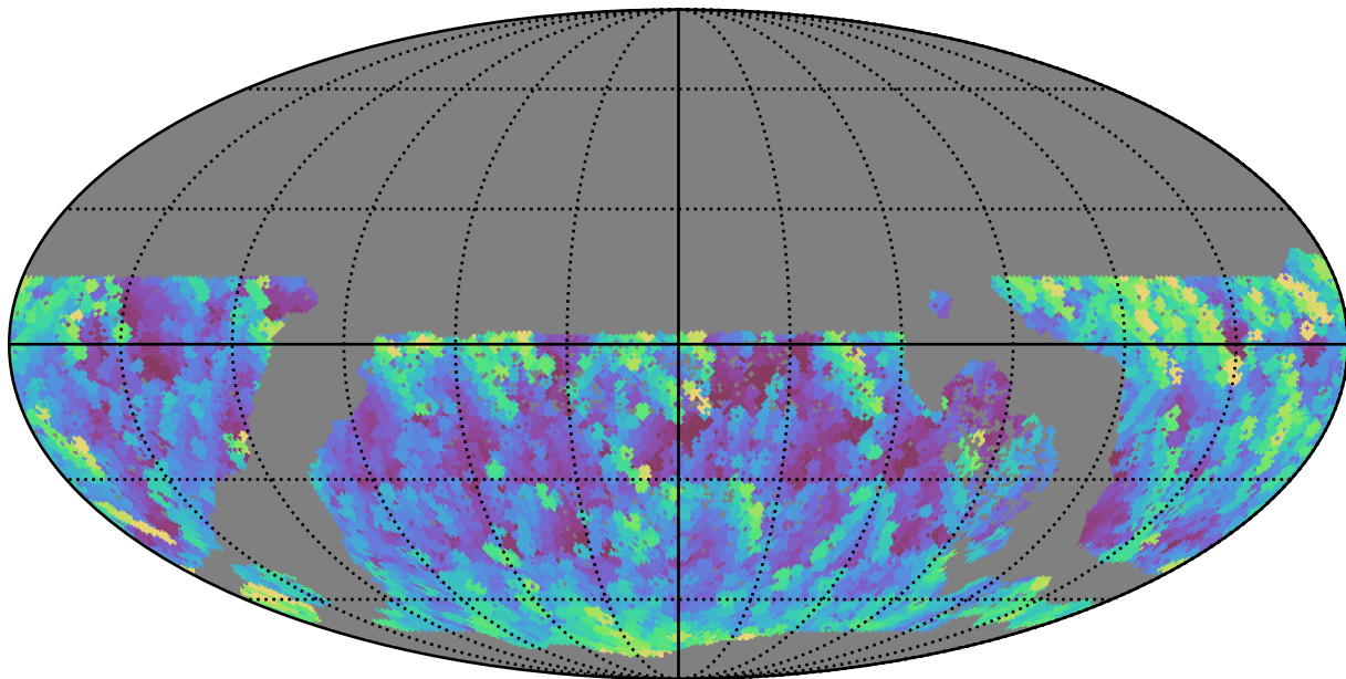
roman_v3.3_10yrs WFD g band: Max airmass
