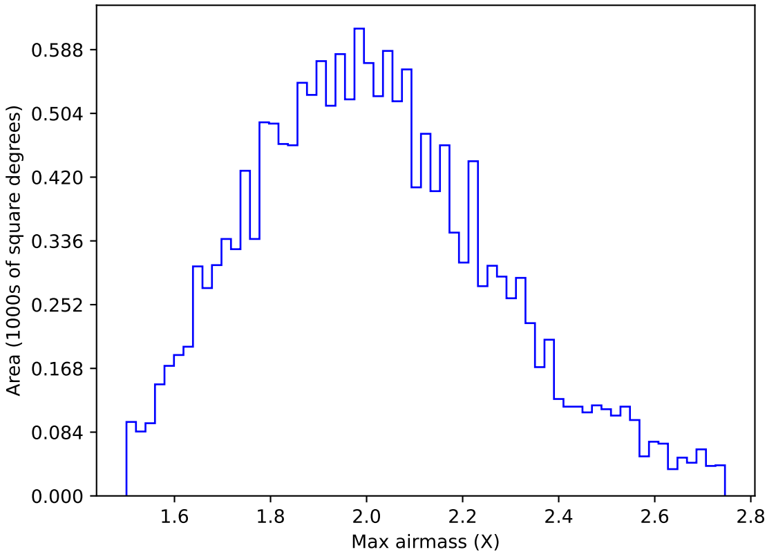
roman_v3.3_10yrs WFD g band: Max airmass
