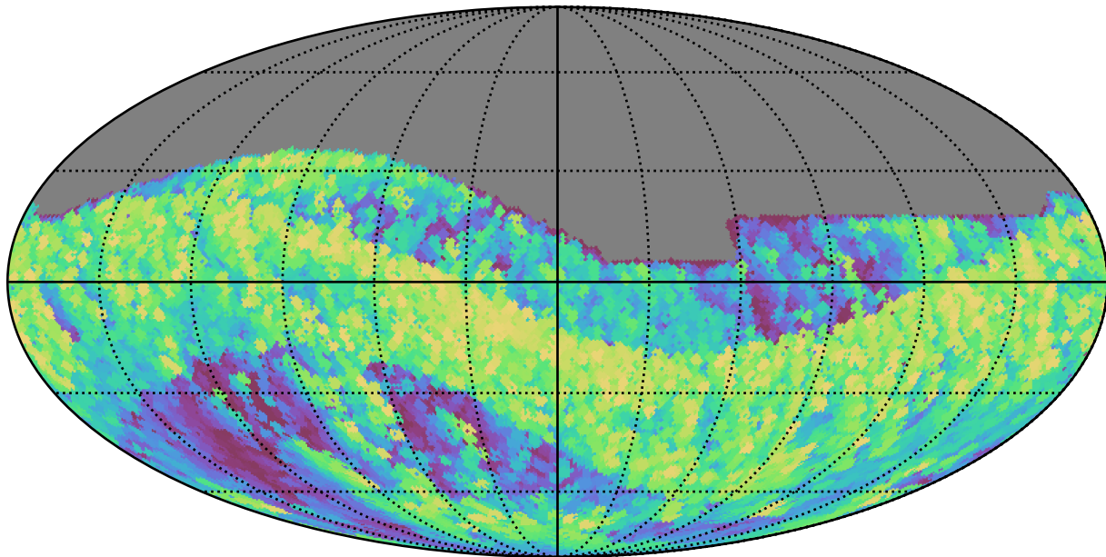
roman_v3.3_10yrs All sky z band: Max airmass
