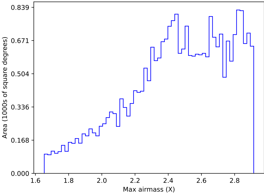
roman_v3.3_10yrs All sky z band: Max airmass
