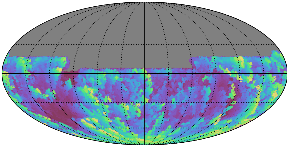
roman_v3.3_10yrs All sky u band: Max airmass
