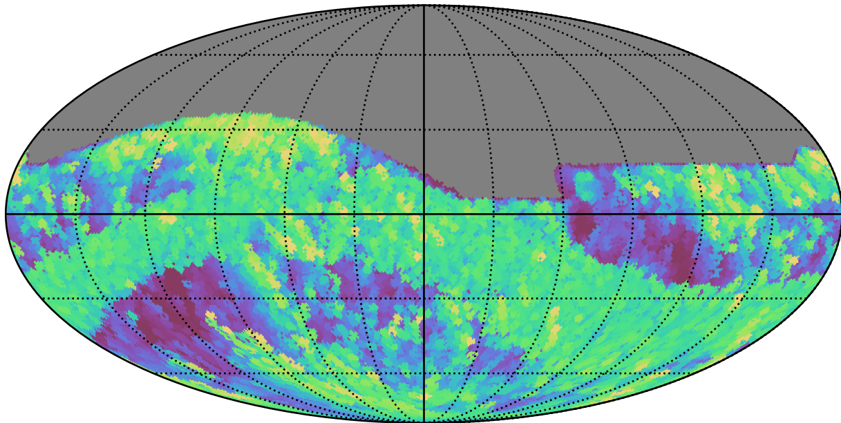
roman_v3.3_10yrs All sky r band: Max airmass
