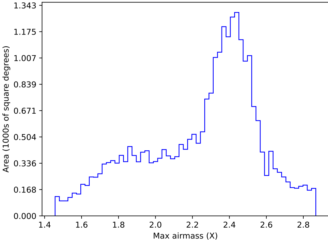
roman_v3.3_10yrs All sky r band: Max airmass
